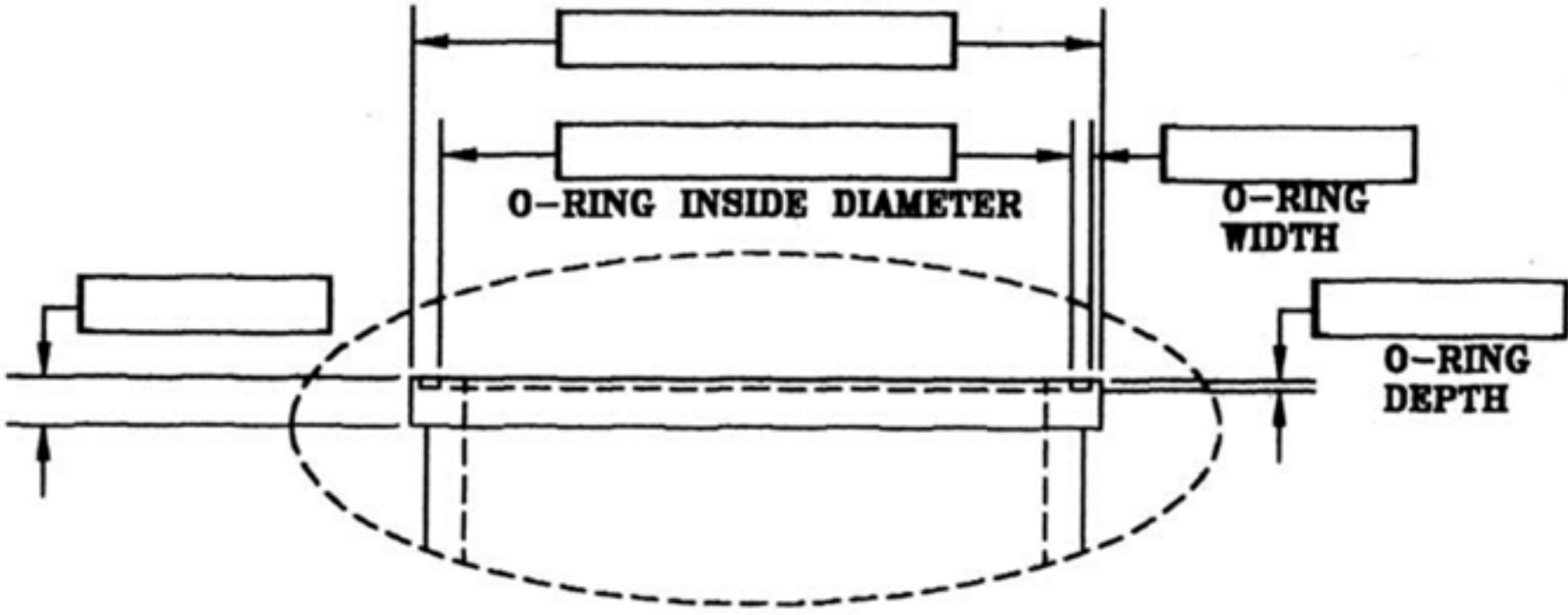
O-RING TYPE SLEEVE (IF APPLICABLE)
